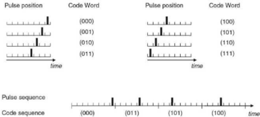
Figure 4-27: 8-PPM Modulation
